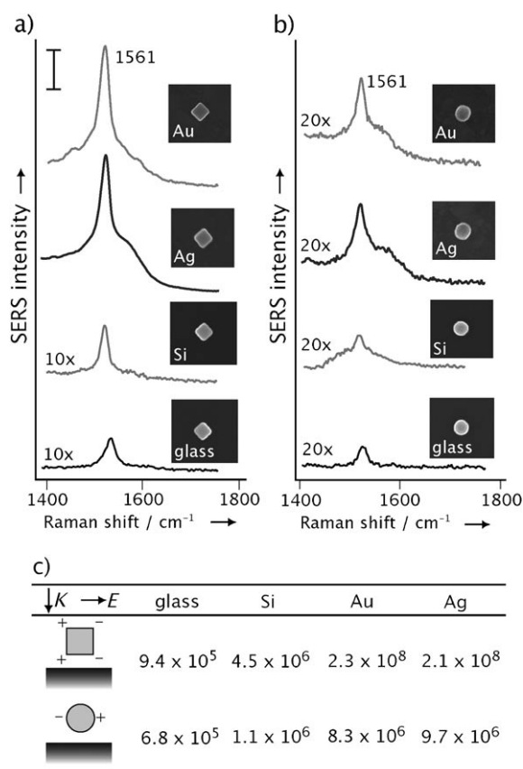
Figure 1. The SERS spectra of 1,4-BDT from: a) nanocubes ( 106 \pm 5 ) nm in edge length and b) nanospheres ( 97 \pm 7 ) nm in diameter, on an Au film, Ag film, Si wafer, and glass cover slip, respectively. The insets show their corresponding SEM images. The scale bar for the SERS spectra is 10 \text{ a.u. mW}^{-1} \text{ s}^{-1} . c) The EFs for single Ag nanocubes and nanospheres, respectively, supported on different substrates. Each value reported in this table represents an average of the data from 40 particles. The cartoon shows propagation and polarization directions of the laser used in this study and simplified distribution of dipolar charges on each type of particle.
