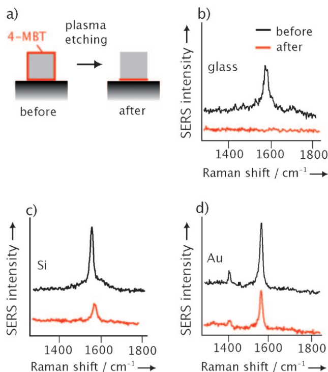
Figure 2. a) Selective removal of 4-MBT molecules (red) from the surface of a Ag nanocube supported on a substrate. Plasma etching with O 2 can remove the exposed molecules on the particle's surface, leaving behind molecules at the nanocube–substrate interface. SERS spectra taken from Ag nanocubes functionalized with 4-MBT (with a peak at 1592 cm -1 ) and then deposited on b) glass, c) Si, and d) on Au microplate substrates. The SERS spectra were recorded from the same nanocube before and after plasma etching.
