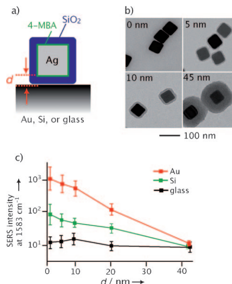
Figure 3. a) Schematic showing how the gap distance ( d ) between a Ag nanocube and its underlying substrate is controlled by the thickness of the SiO 2 shell (blue). The nanocube was functionalized with SERS-active 4-MBA (green) prior to coating with SiO 2 . b) TEM images of Ag nanocubes coated with SiO 2 shells of 0, 5, 10, and 45 nm, respectively, in thickness. c) Plots of SERS peak intensity as a function of thickness for the SiO 2 shell. The peak intensities at 1583 cm -1 were recorded for the 4-MBA molecules on single nanocubes supported on Au film, Si wafer, and glass substrates, respectively.
