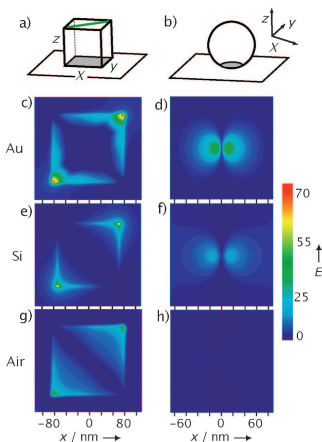
Figure 4. Simulated E-field enhancements for a Ag nanocube or nanosphere. a, b) Coordination systems for calculating the E-field enhancement distribution of a nanocube and nanosphere, respectively, positioned 2 nm above a substrate. The gray region represents the plane plotted in the simulations and is 1 nm above the underlying substrate. For nanocubes, the polarization was along the green line. The E-field enhancement distributions calculated using the DDA method for: nanocubes c) on Au, e) on Si, and g) in air; as well as for nanospheres d) on Au, f) on Si, and h) in air.
